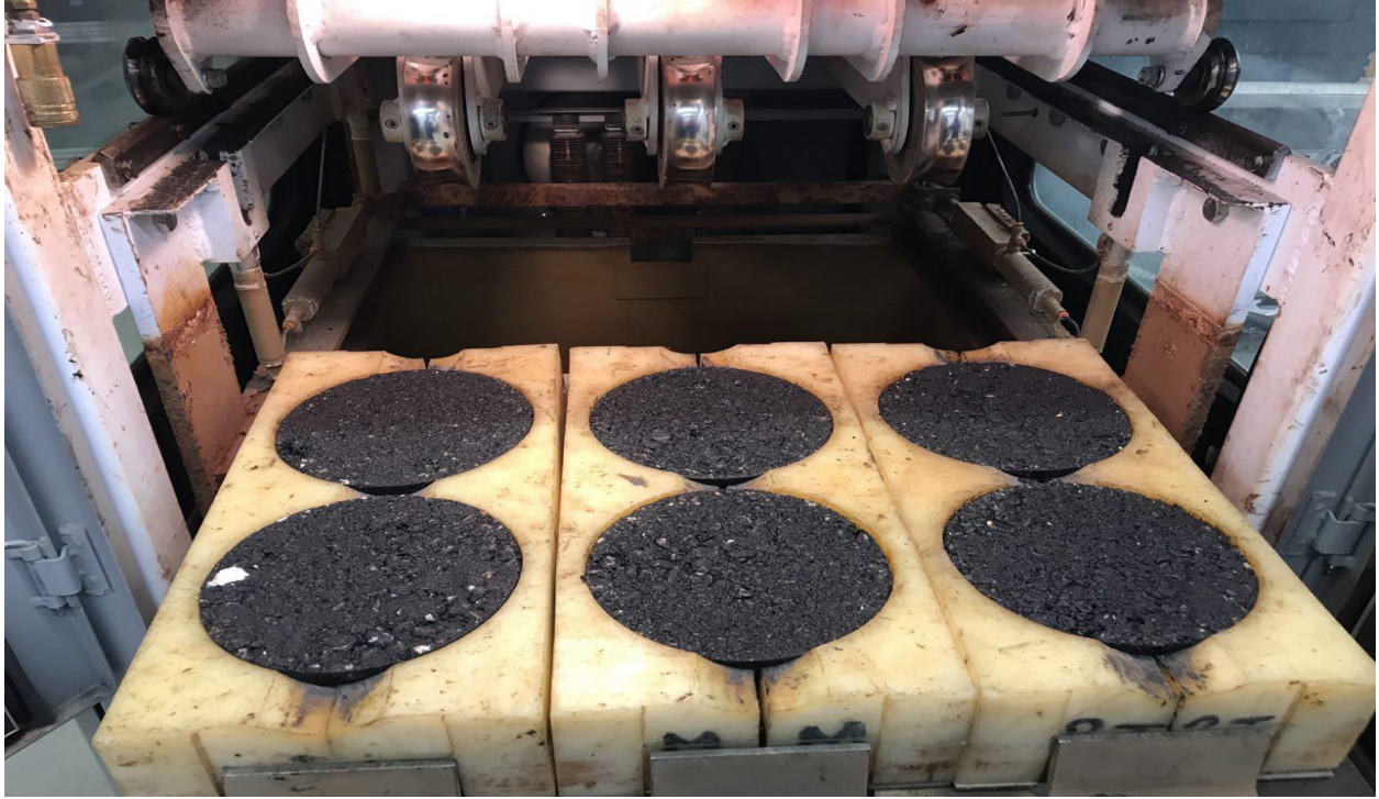
Figure 4.8. APA specimen layout before test
